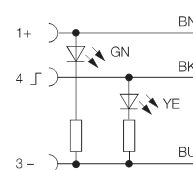
With 2 LED lights, suitable for PNP sensor
